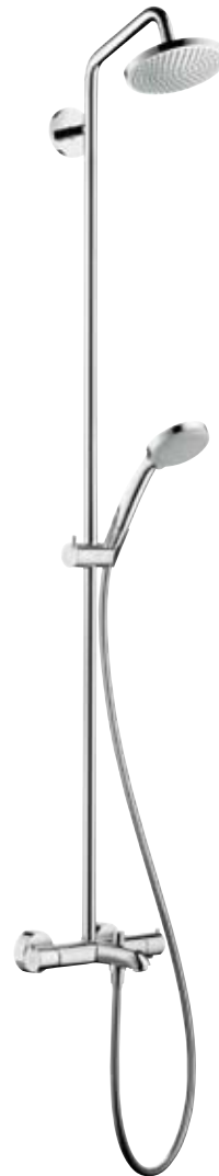
Croma® 220 Showerpipe for the bath with swivelling overhead shower Croma 220 1jet (16 l/min), Croma 100 Vario hand shower (15 l/min), Ecostat Comfort bath spout (20 l/min), shower arm 400 mm Height of the riser pipe can be reduced # 27223,-000
